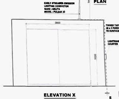
ELEVATION X
