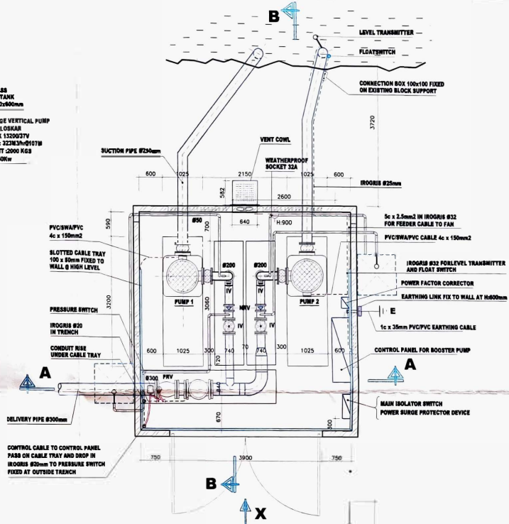
PLAN
